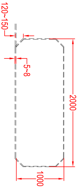
LOOP CUTTING DETAIL
